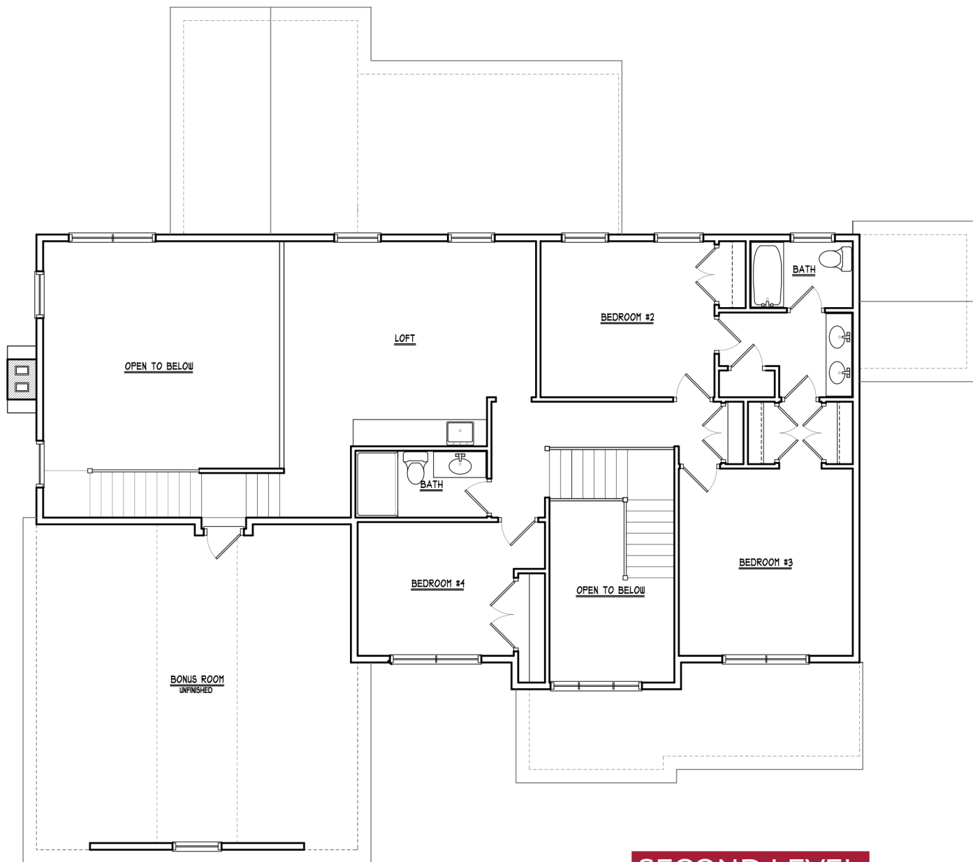
SECOND LEVEL 1,750 SQ FT
