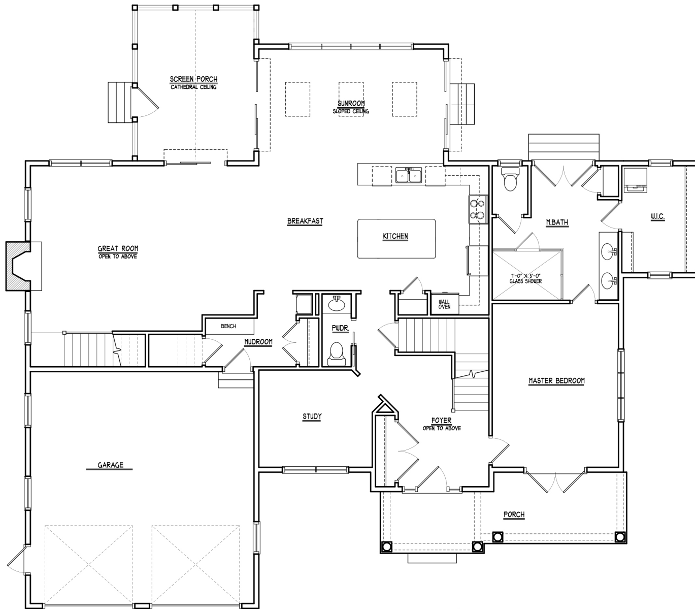
MAIN LEVEL 2,090 SQ FT
